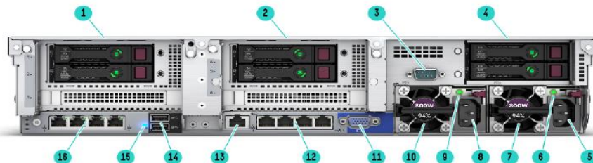
Rear View – With optional FlexLOM, Rear drives and Serial port shown.
